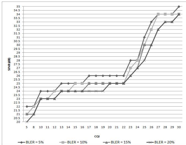
Fig. 3. SINR vs CQI in case of Good Channel
