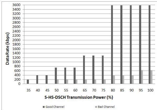
Fig. 5. Data Rate vs S-HS-DSCH Transmission Power, with BLER 10%
