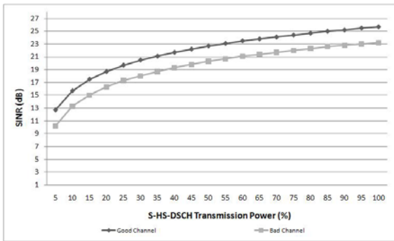
Fig. 2. SINR vs S-HS-DSCH Transmission Power
