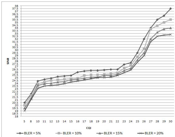
Fig. 4. SINR vs CQI in case of Bad Channel
