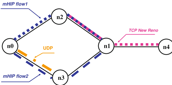
Fig. 1. 2-path simulation model
