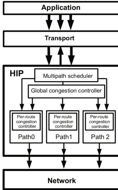
Fig. 3. Two-level multipath congestion control
