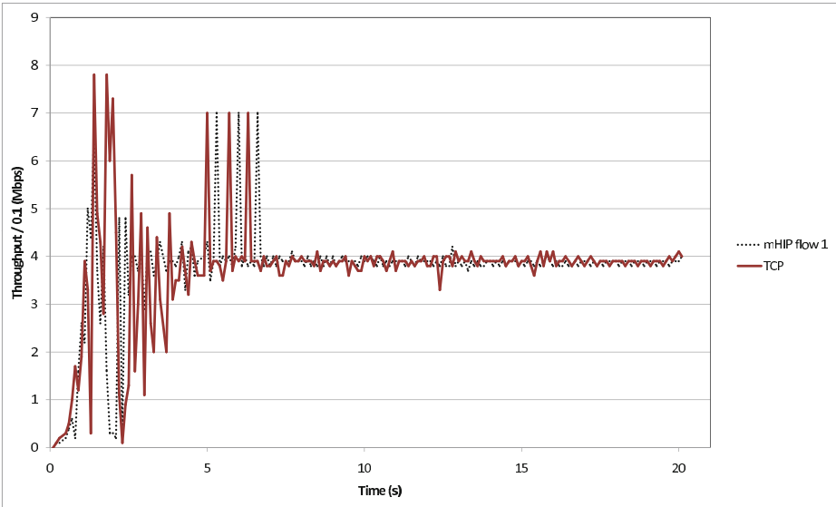
Fig. 5. mHIP flow 1 friendly coexists with TCP New Reno flow
