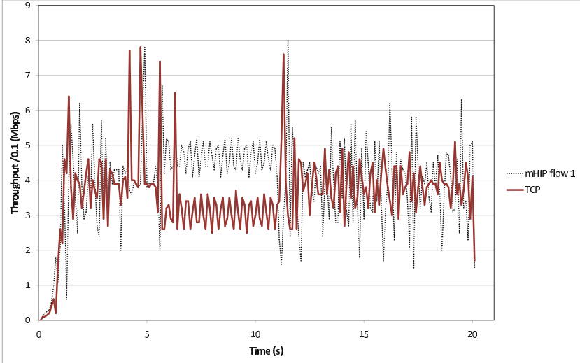
Fig. 2. mHIP flow competes with TCP New Reno flow in Path1
