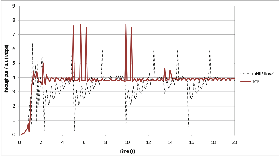
Fig. 4. mHIP flow controlled by the proposed twofold multipath congestion control is suppressed by TCP
