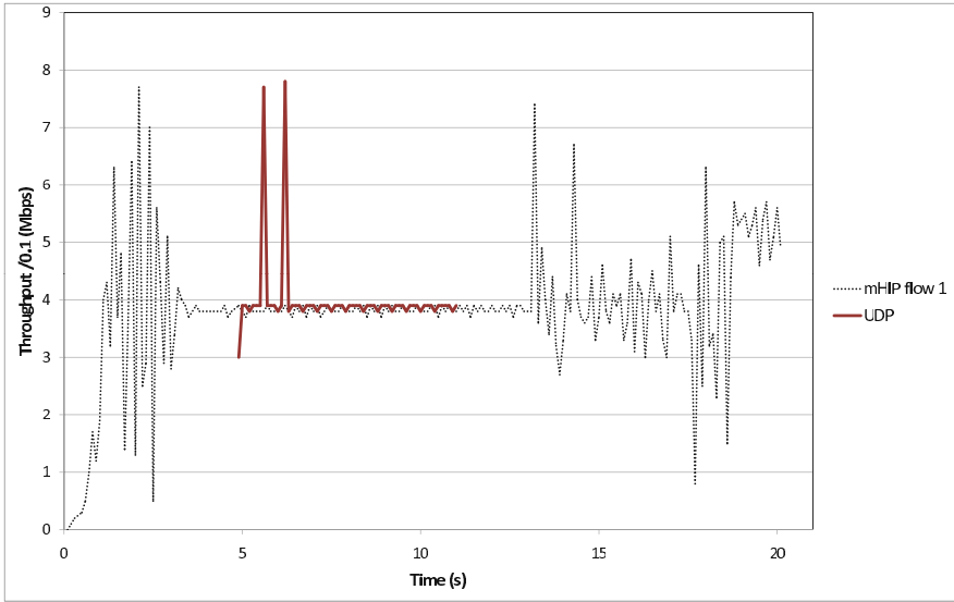
Fig. 6. mHIP flow 2 competes almost friendly with UDP cross-traffic
