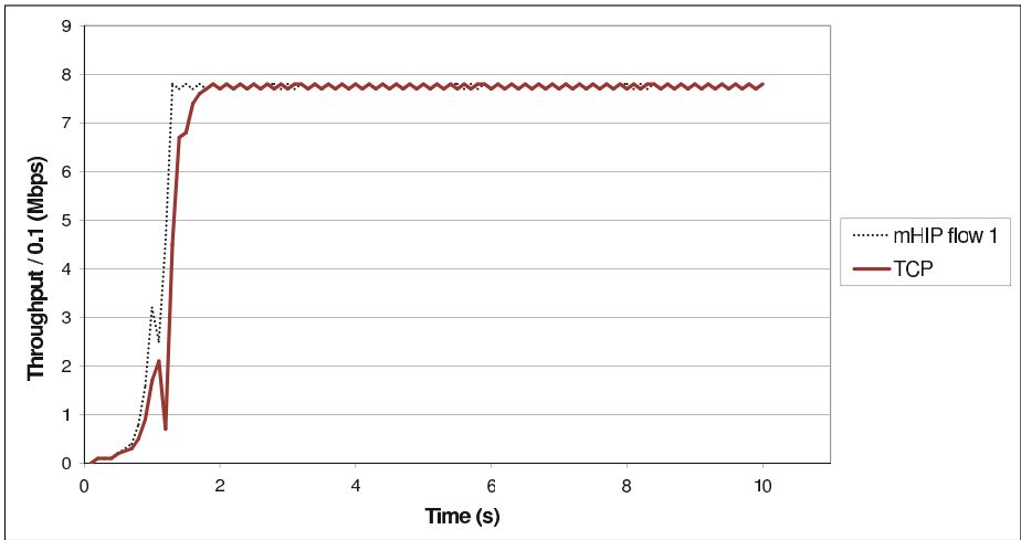
Fig. 7. Testing TCP-compatibility and equivalence of mHIP
