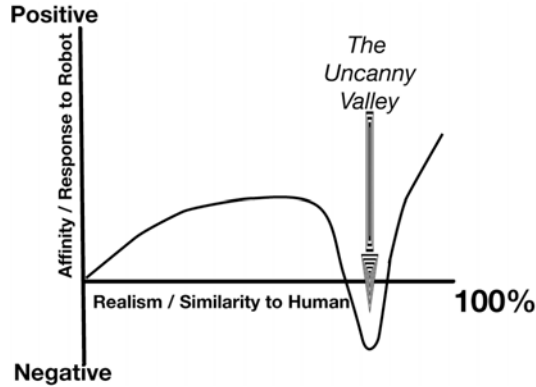
Fig. 1. Simplified diagram showing the hypothesized relationship between affinity and realism with the uncanny valley appearing as a negative response as one approaches total realism
