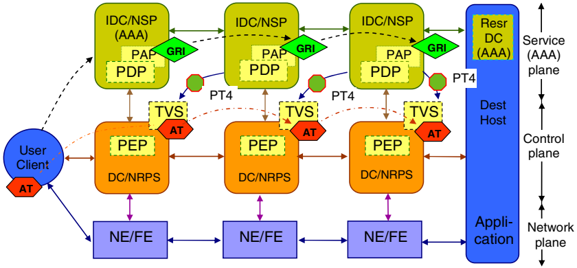
Fig. 1. Components involved in multidomain network resource provisioning. CRP stages reservation, deployment and access are presented by the flows correspondingly GRI (forward from the user to the resource), pilot tokens PT4 (backward), and access tokens AT (forward).
