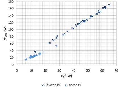
Fig. 2. Power consumption of Desktop and Laptop PC's
