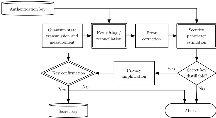
Fig. 1. Flow chart of the stages of a quantum key distribution protocol. Stages with double lines require classical authentication.
