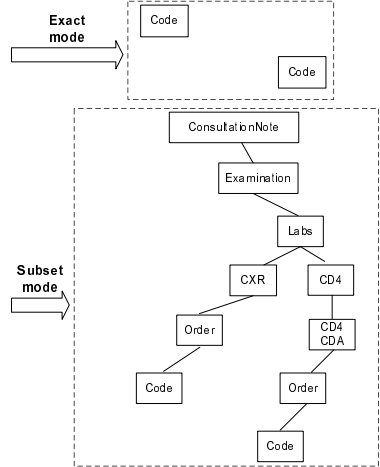
(c) Property Match
