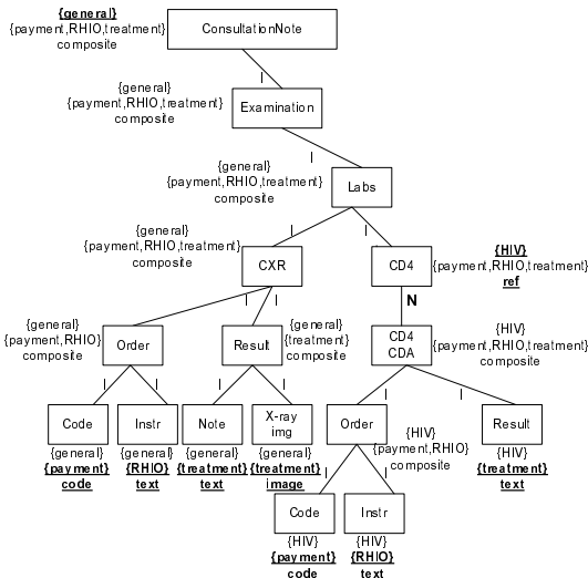
(b) Property Labeling and Propagation
