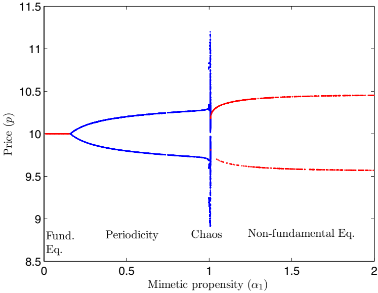
Fig. 4. Bifurcation diagram with \alpha_2 = 0.2 and \alpha_3 = 0.5
