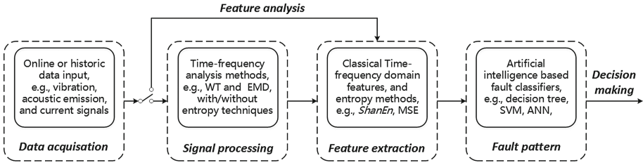
Fig. 1. Data flow of fault diagnosis of rotating machinery based entropy methods.
