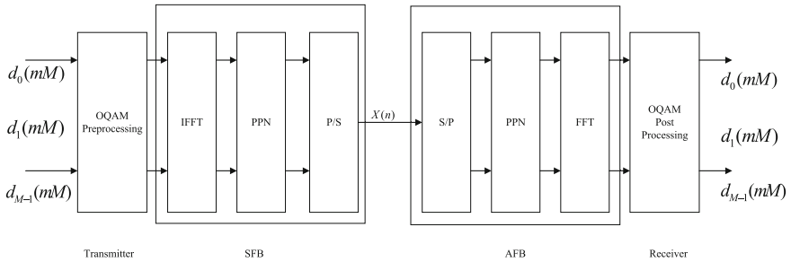
Fig. 2. The basic architecture of the FBMC system.
