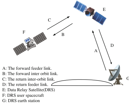
Fig. 1. Data relay satellite system
