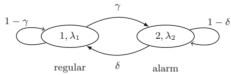
Fig. 3. The state diagram of an IED traffic generation modeled with an MMPP.
