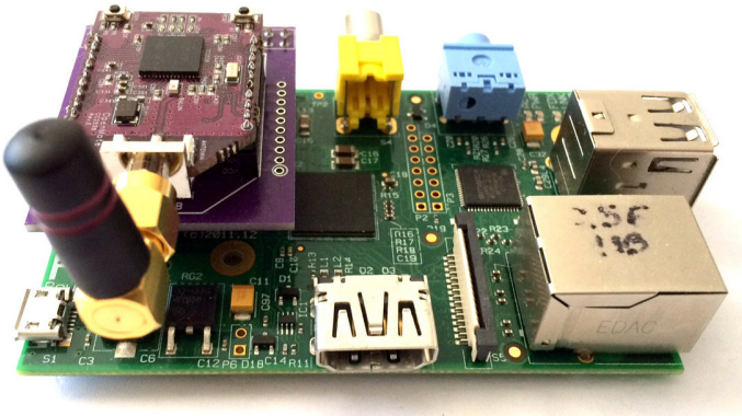
Fig. 3. The Raspberry Pi adapter for the OpenMote.
