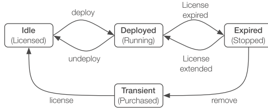
Fig. 1. IoT Application lifecycle
