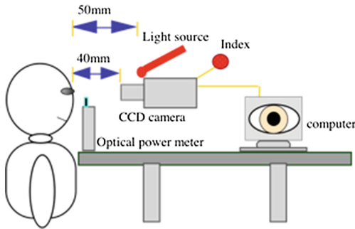
Fig. 1. Light reflex measuring system
