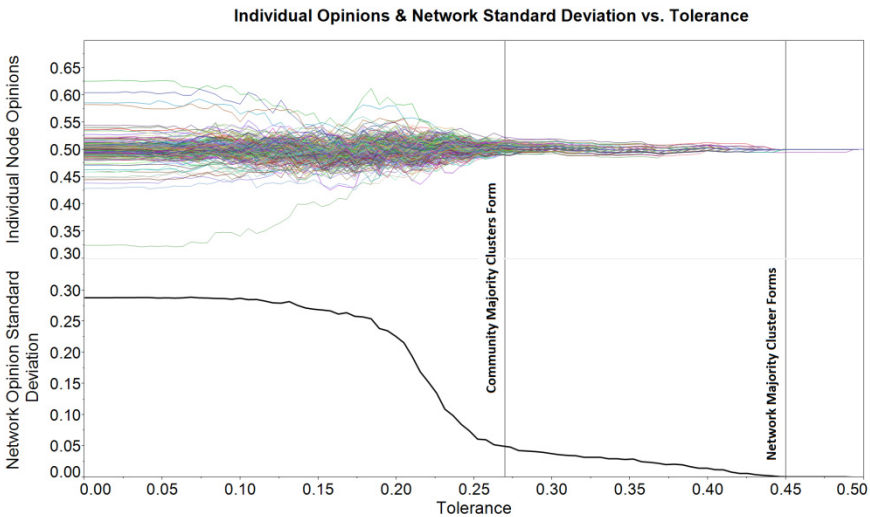
Fig. 5. Individual node opinions for the entire network plotted relative to tolerance values (above) are shown in the context of the standard deviation of opinion for the entire network (below). The individual node opinions come into consensus at tolerance \sim 0.45 indicating the formation of the single majority-opinion network cluster.
