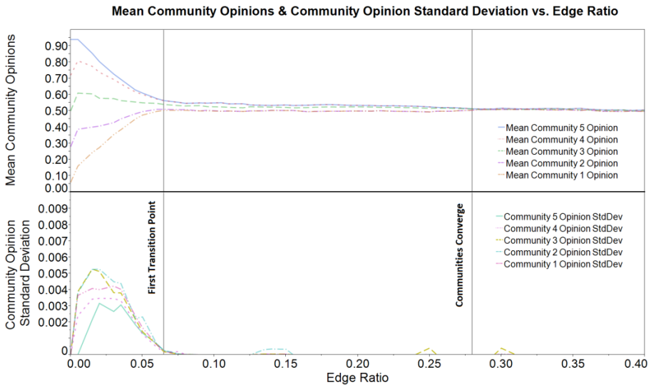
Fig. 7. Effect of between-community to within-community edge ratio on mean community opinion and standard deviation. The mean community opinion (upper) plot shows consensus among the five communities commencing at \sim 0.065 with near complete consensus at \sim 0.28 . The standard deviation (lower) plot shows the communities at consensus amongst themselves at the onset.
