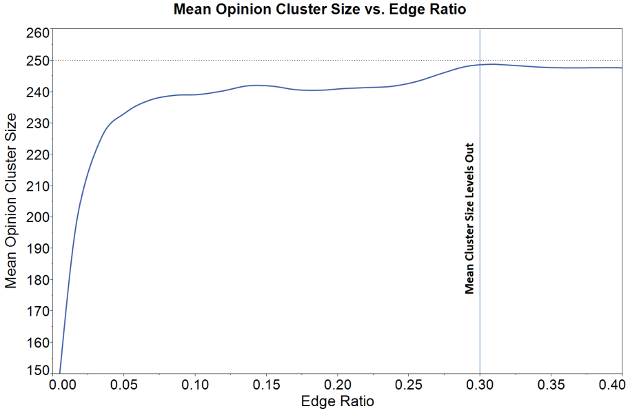
Fig. 9. Effect of between-community to within-community edge ratio on mean opinion cluster size. Mean cluster size can be seen to level out in the vicinity of an edge ratio of \sim 0.30 , very near the point at which community opinions converged in the previous results (0.28).
