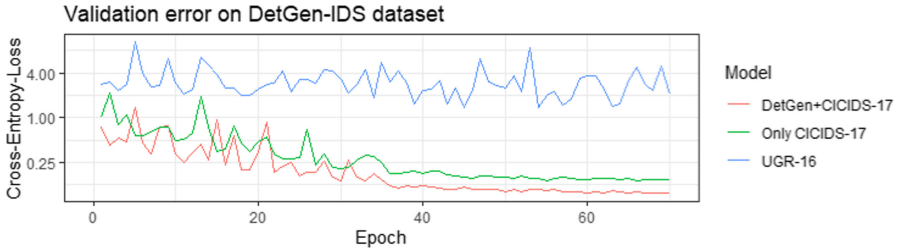
Fig. 8. Validation errors of LSTM-model [4] on DetGen-IDS data. (Color figure online)
