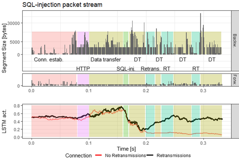
Fig. 3. LSTM-classification output in dependence of connection phases. (Color figure online)
