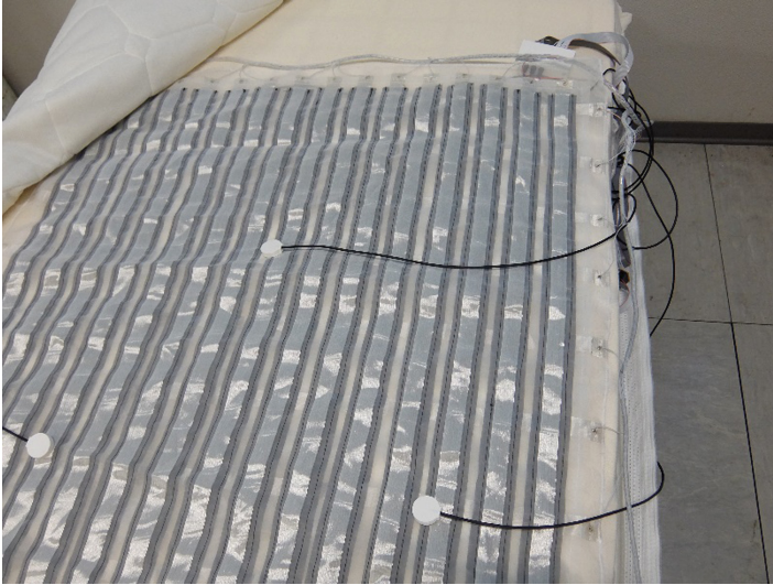
Fig. 2. Position of accelerometers (white dots) over the pressure matrix.
