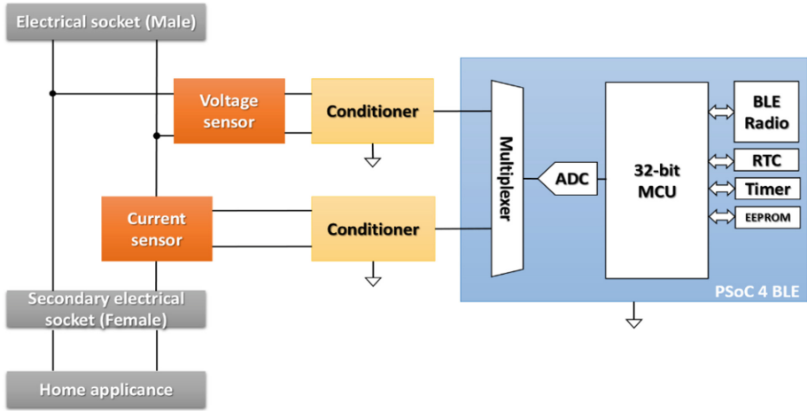
Fig. 3. Block diagram of the monitoring device.
